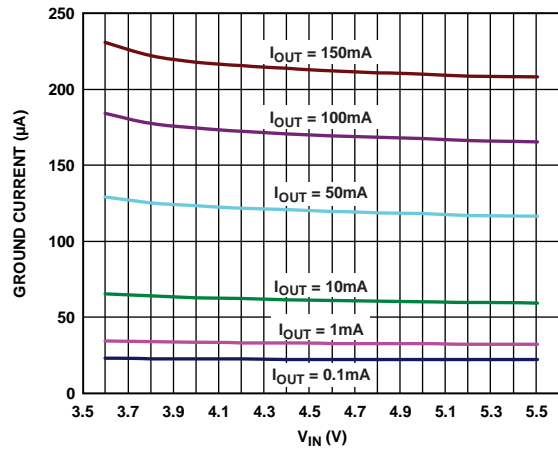
Figure 10. Ground Current vs. Input Voltage ( V_{IN} )
