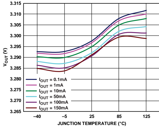
Figure 5. Output Voltage ( V_{OUT} ) vs. Junction Temperature
